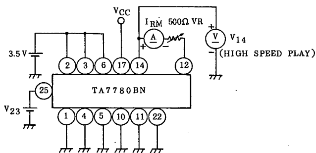
TEST CIRCUIT 5 : V_{14(High\ Speed\ PLAY)}
