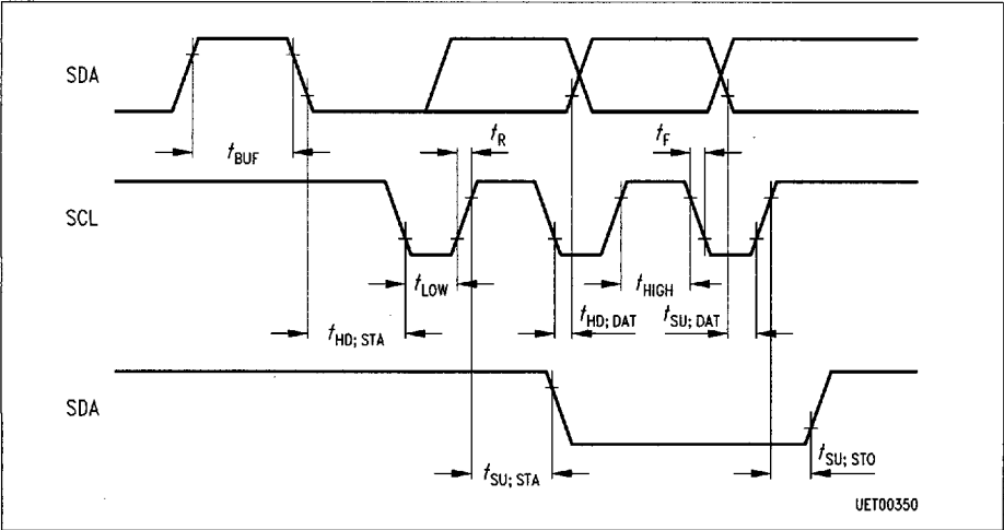
Figure 2 Timing Conditions for the I²C Bus (high-speed mode)
