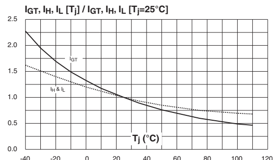
Figure 2. Relative variation of gate trigger current, holding current and latching current versus junction temperature (typical values)
