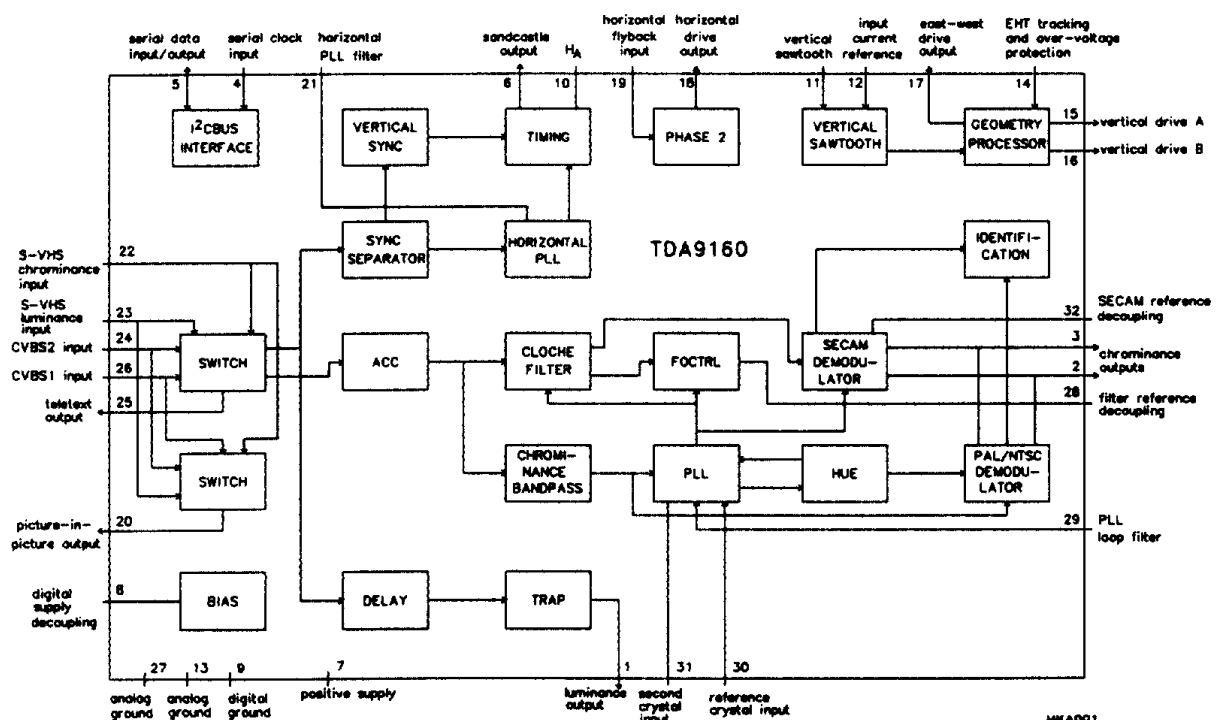
Fig.1 Block diagram.
