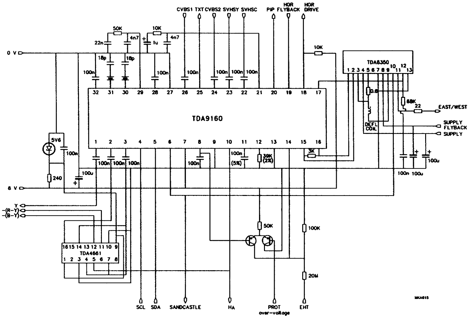
Fig.17 Application diagram.
