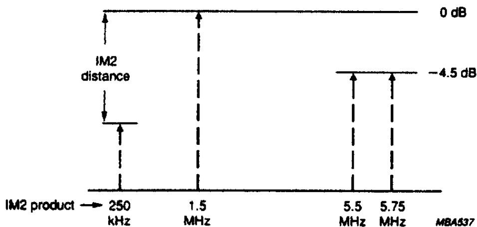
Fig.3 IM2 product.
