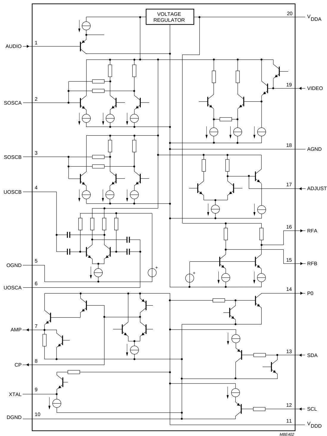
Fig.6 Pin equivalent circuit for each pin.
