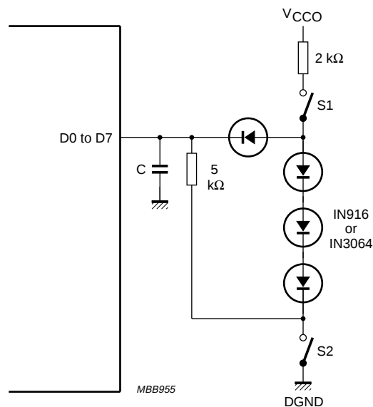
Fig.6 Load circuit for timing measurement; 3-state outputs ( \overline{\text{CE}} : f_i = 1 \text{ MHz} ; V_{VI} = 3 \text{ V} ); see Table 3.
