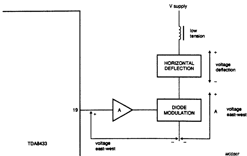
Fig.9 Application diagram for driving the diode modulator.
