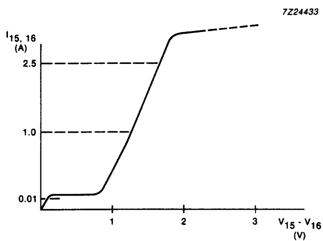
Fig.11 Saturation curve.
