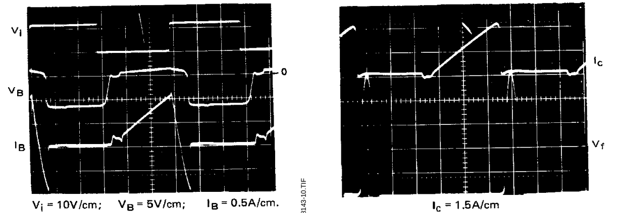
Figure 8 : Signal Diagrams of the Driver Circuits
