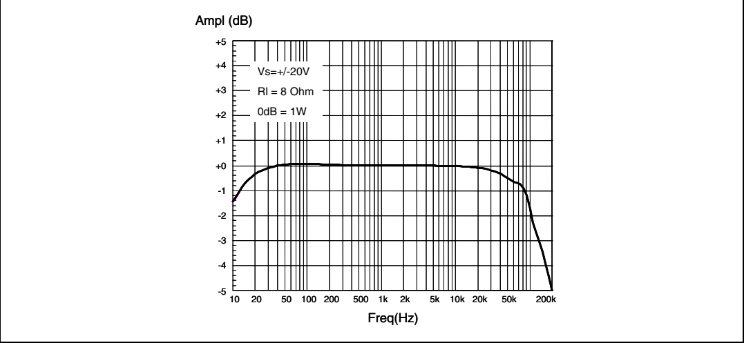
Figure 4. Frequency response
