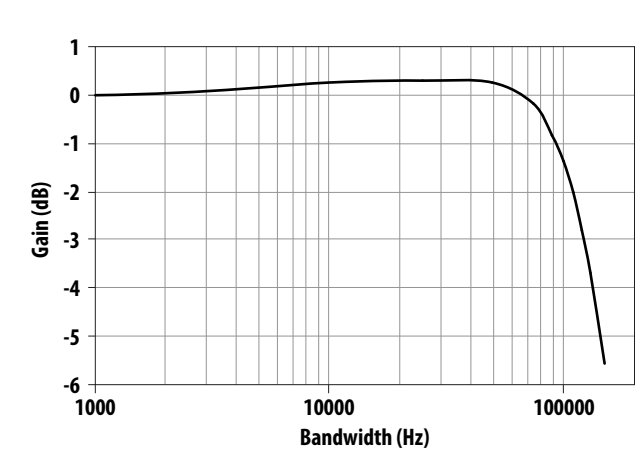
Figure 14: Frequency Response
