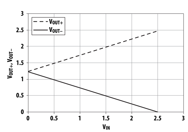
Figure 13: VIN vs. VOUT+, VOUT-
