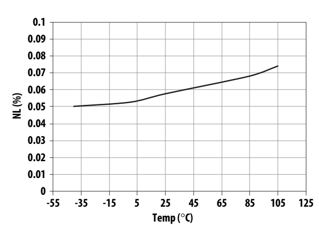
Figure 11: Non-Linearity vs. Temperature
