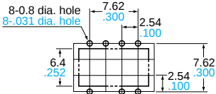
PC board pattern (BOTTOM VIEW)
