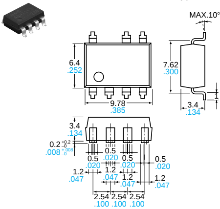
Surface mount terminal type
