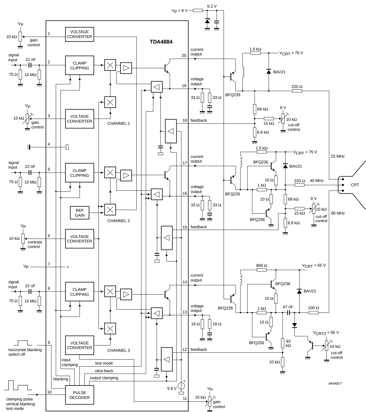
Fig.1 Block diagram and basic application circuit for DC and AC coupling.
