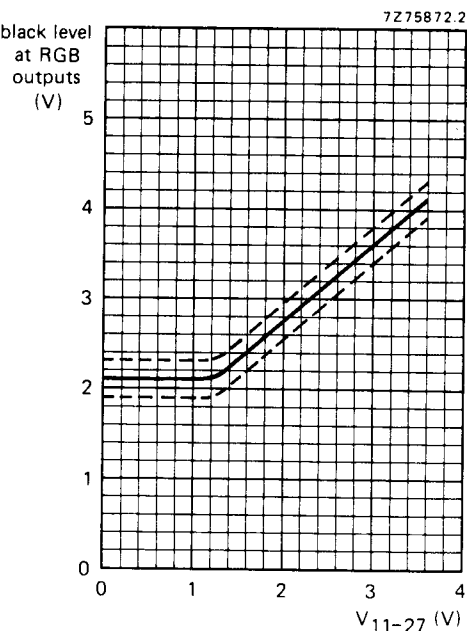
Fig. 5 Brightness control voltage range.
