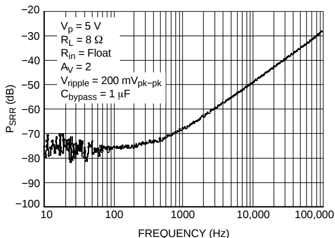
Figure 13. \text{PSRR} @ V_p = 5\text{ V}
