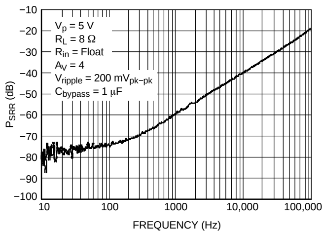
Figure 15. \text{PSRR} @ V_p = 5\text{ V}
