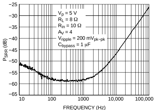
Figure 14. \text{PSRR} @ V_p = 5\text{ V}
