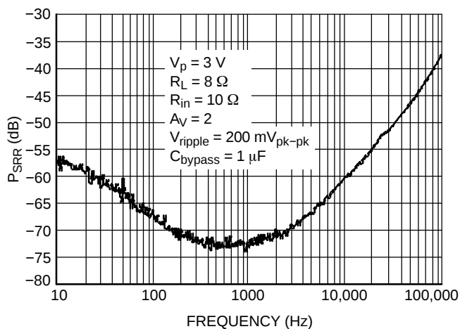
Figure 16. \text{PSRR} @ V_p = 3\text{ V}
