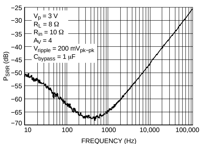
Figure 18. \text{PSRR} @ V_p = 3\text{ V}
