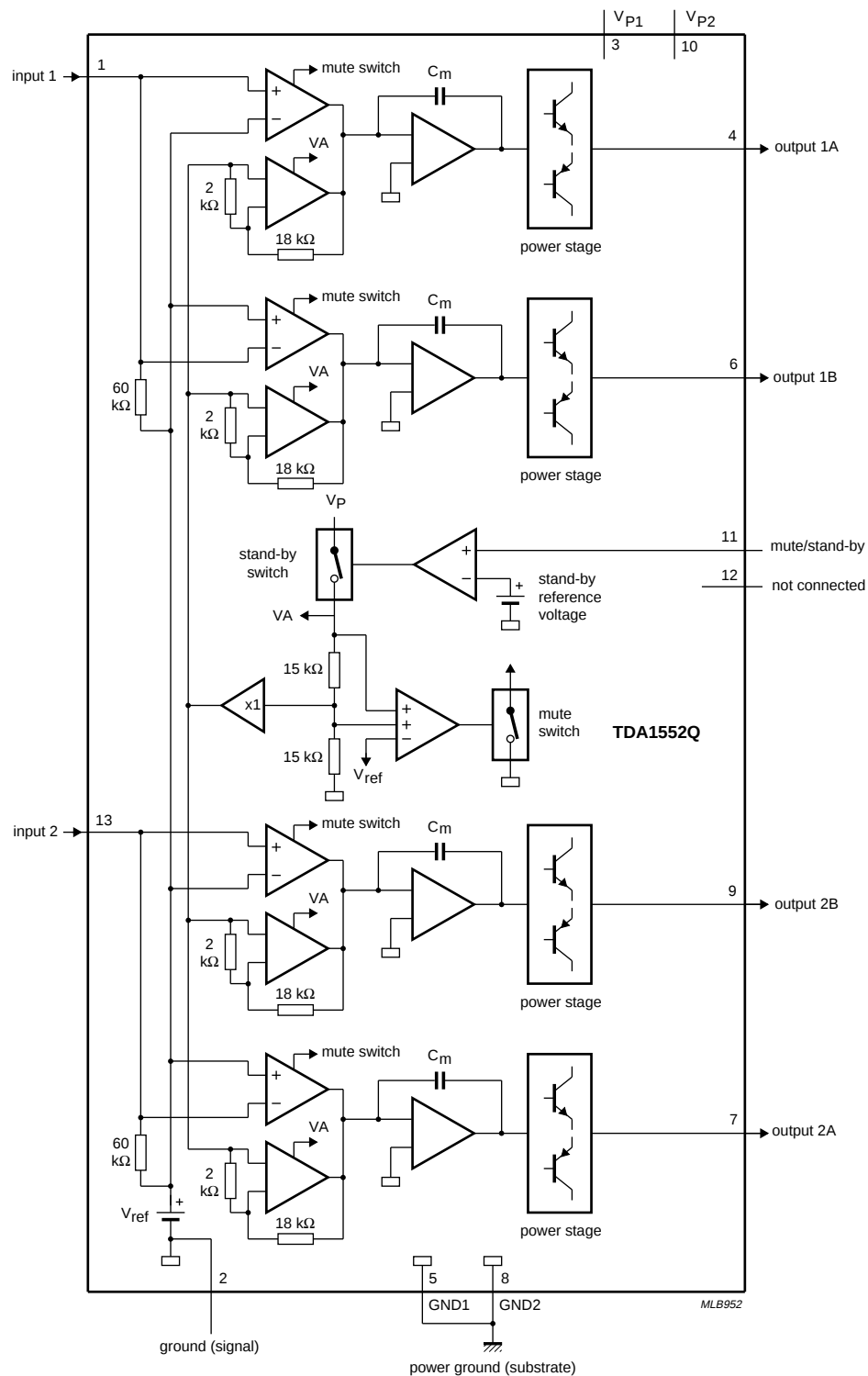
Fig.1 Block diagram.
