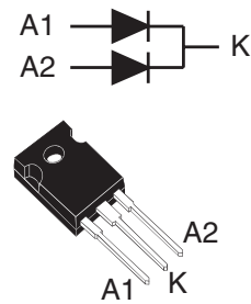
TO-247 STTH6002CW
