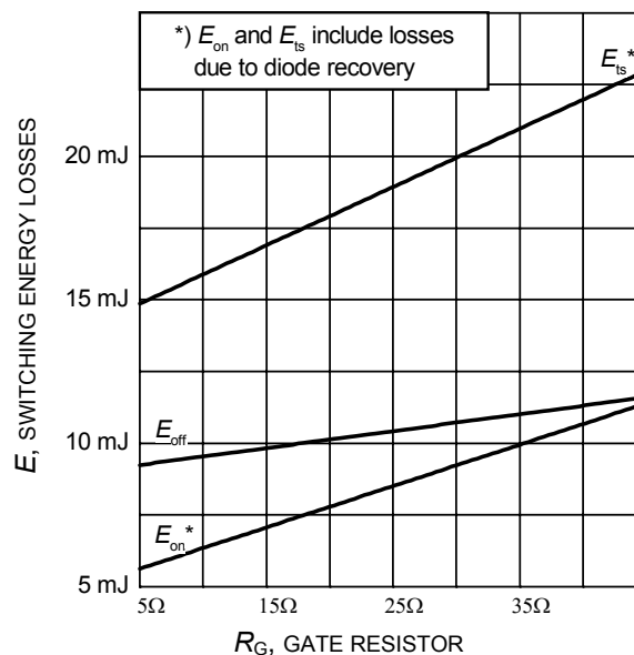
Figure 14. Typical switching energy losses as a function of gate resistor (inductive load, T_J=150^\circ\text{C} , V_{CE}=600\text{V} , V_{GE}=0/15\text{V} , I_C=60\text{A} , Dynamic test circuit in Figure E)
