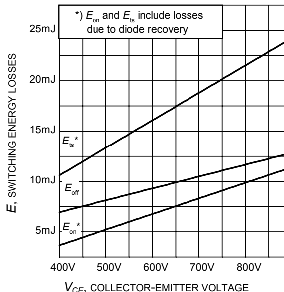
Figure 16. Typical switching energy losses as a function of collector emitter voltage (inductive load, T_J=150^\circ\text{C} , V_{GE}=0/15\text{V} , I_C=60\text{A} , R_G=10\Omega , Dynamic test circuit in Figure E)
