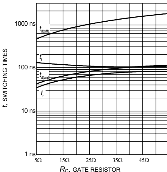
Figure 10. Typical switching times as a function of gate resistor (inductive load, T_J=150^\circ\text{C} , V_{CE}=600\text{V} , V_{GE}=0/15\text{V} , I_C=60\text{A} , Dynamic test circuit in Figure E)
