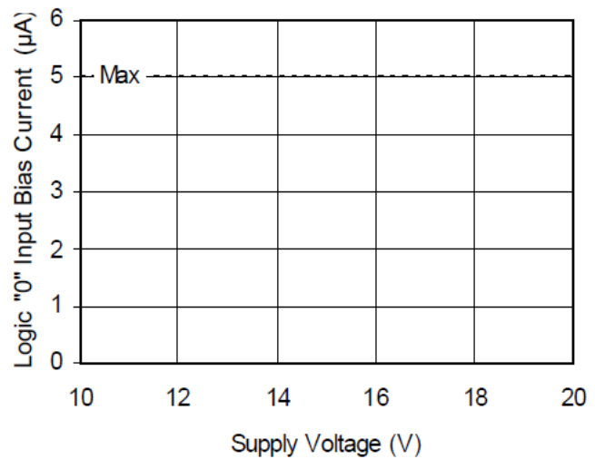
Figure 16B. Logic "0" Input Bias Current vs. Voltage
